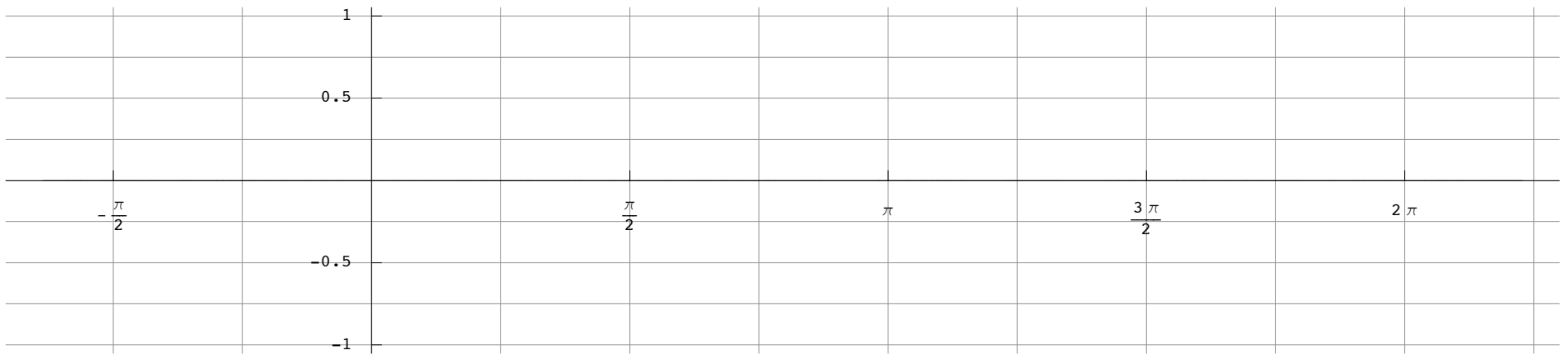
Graph of the tangent line slopes for f(x) = \sin x
