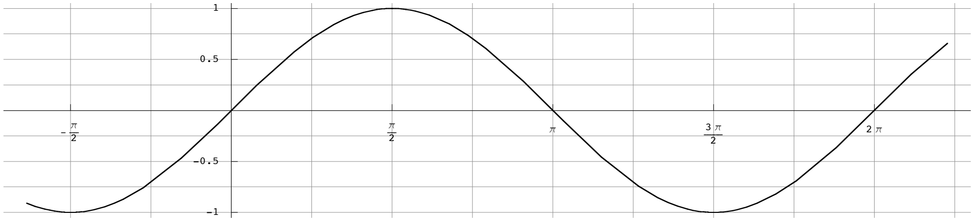
Graph of f(x) = \sin x
