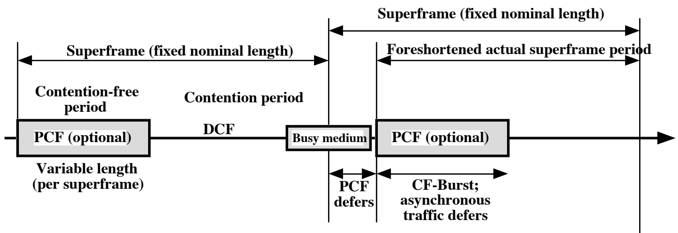
(b) PCF Superframe Construction
